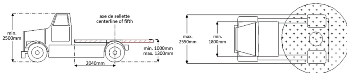
Dessin / Drawing 290-3.17.1
