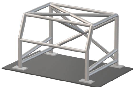
Dessin / Drawing 290-2.9.1
