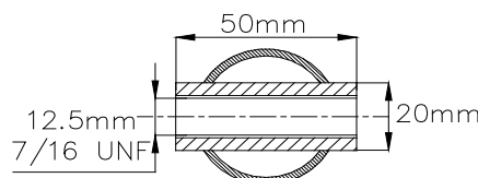
Dessin / Drawing 253-67
