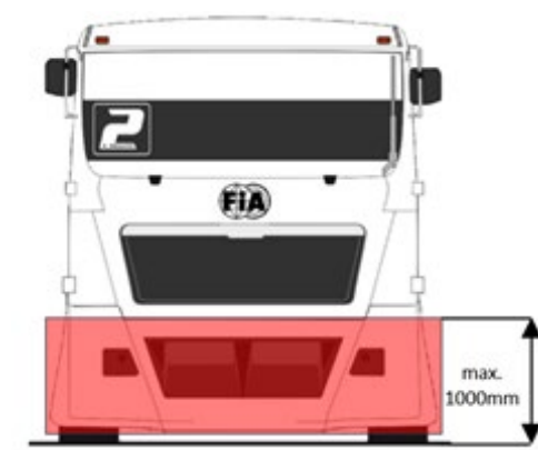
Dessin / Drawing 290-3.17.2.2
