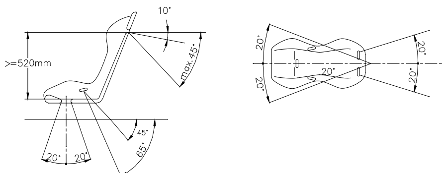
Dessin / Drawing 253-61
